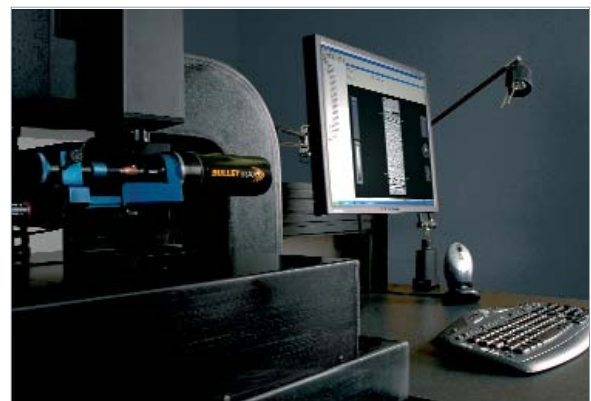
Forensic Technology's 3D Bullet Imaging Station, BulletTRAX-3D.
